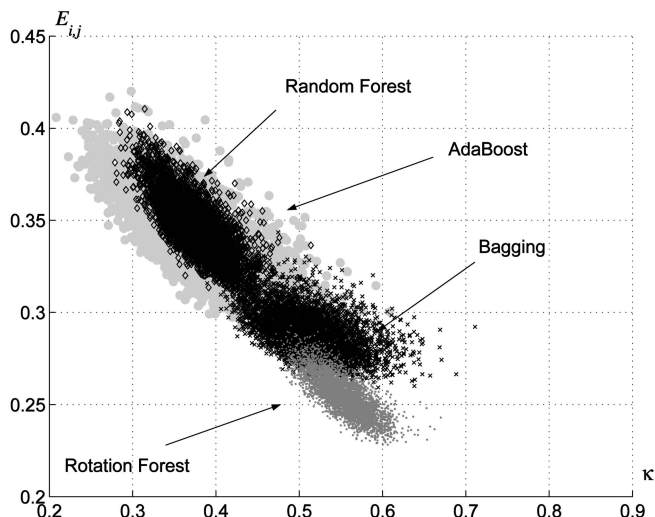
Fig. 8. Kappa-error diagrams for the waveform data set.
