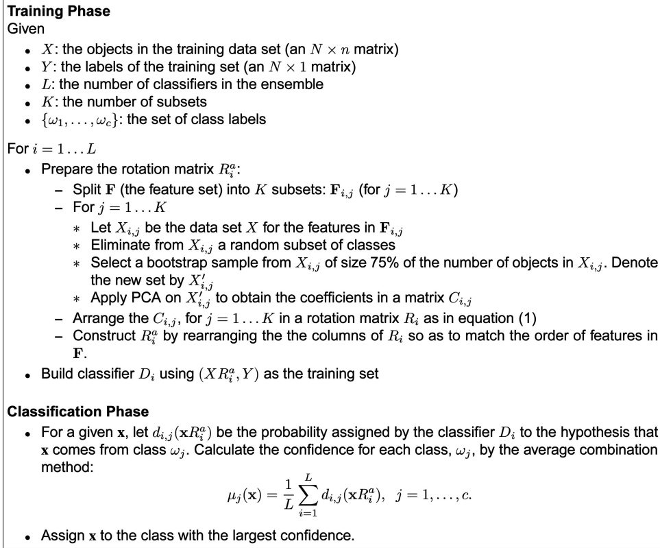
Fig. 1. Pseudocode of the Rotation Forest ensemble method.
