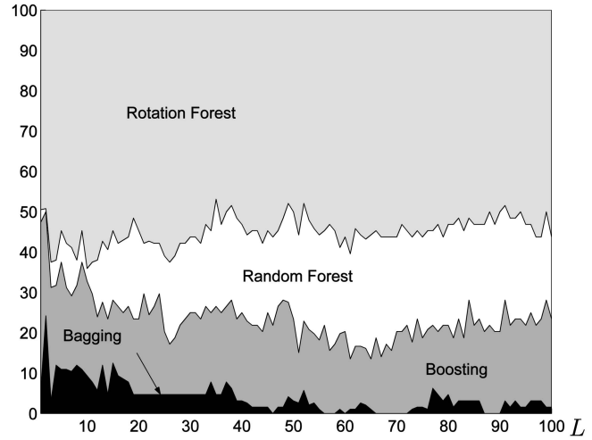
Fig. 3. Percentage diagram for the four studied ensemble methods with unpruned J48 trees.
