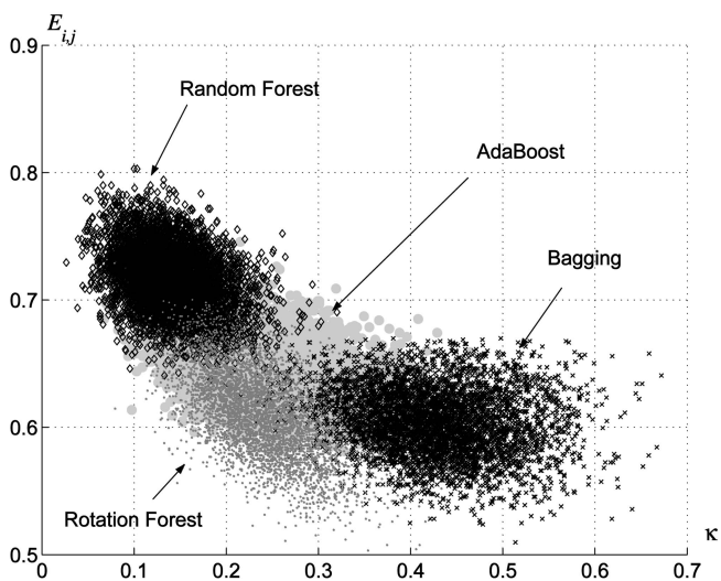
Fig. 7. Kappa-error diagrams for the vowel-n data set.
